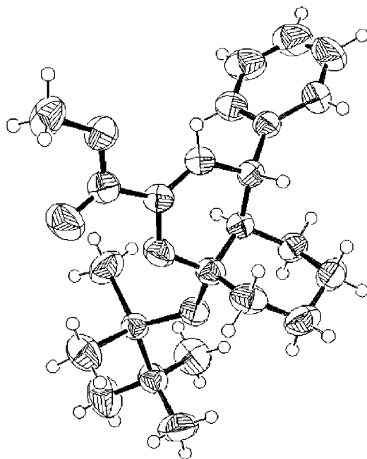
Figure 1. X-ray crystal structure analysis of adduct 3h
