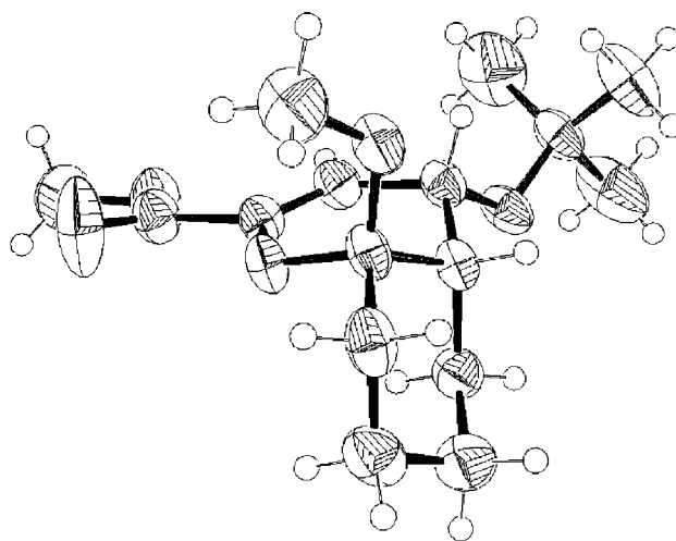
Figure 3. X-ray crystal analysis of adduct 4q
