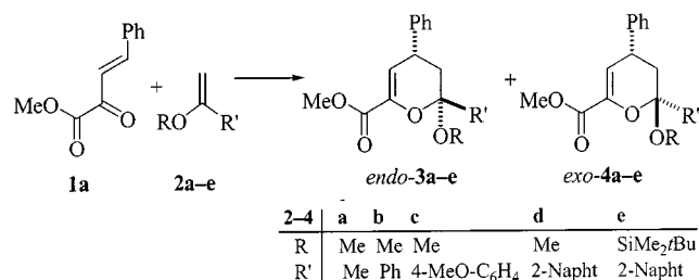
Scheme 2. Conditions: Eu(fod) 3 (5 mol %), reflux
