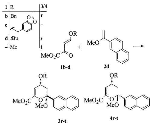
Scheme 10. Conditions: A: \text{Eu}(\text{fod})_3 (5 mol %), reflux; B: \text{SnCl}_4 (5 mol %), \text{CH}_2\text{Cl}_2 , -78 °C, 1–2 h
