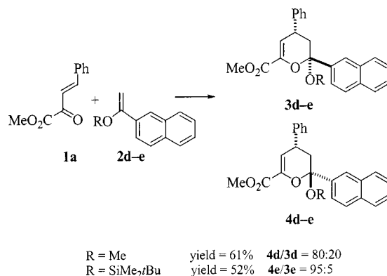
Scheme 6. Conditions: SnCl 4 (9 mol %), CH 2 Cl 2 , 0 °C, 3 h
