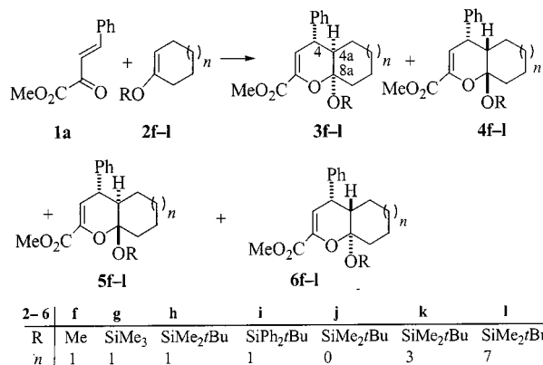
Scheme 3. Conditions: A: Eu(fod) 3 (5 mol %), reflux; B: catalyst, CH 2 Cl 2 , –78 °C, 0.5–1 h
