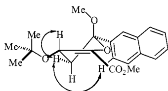
Figure 4. Observed NOE enhancements for 4s
