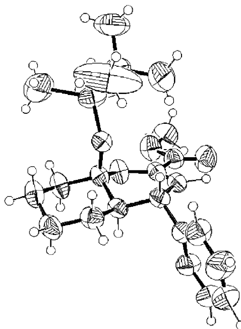
Figure 2. X-ray crystal analysis of adduct 5h
